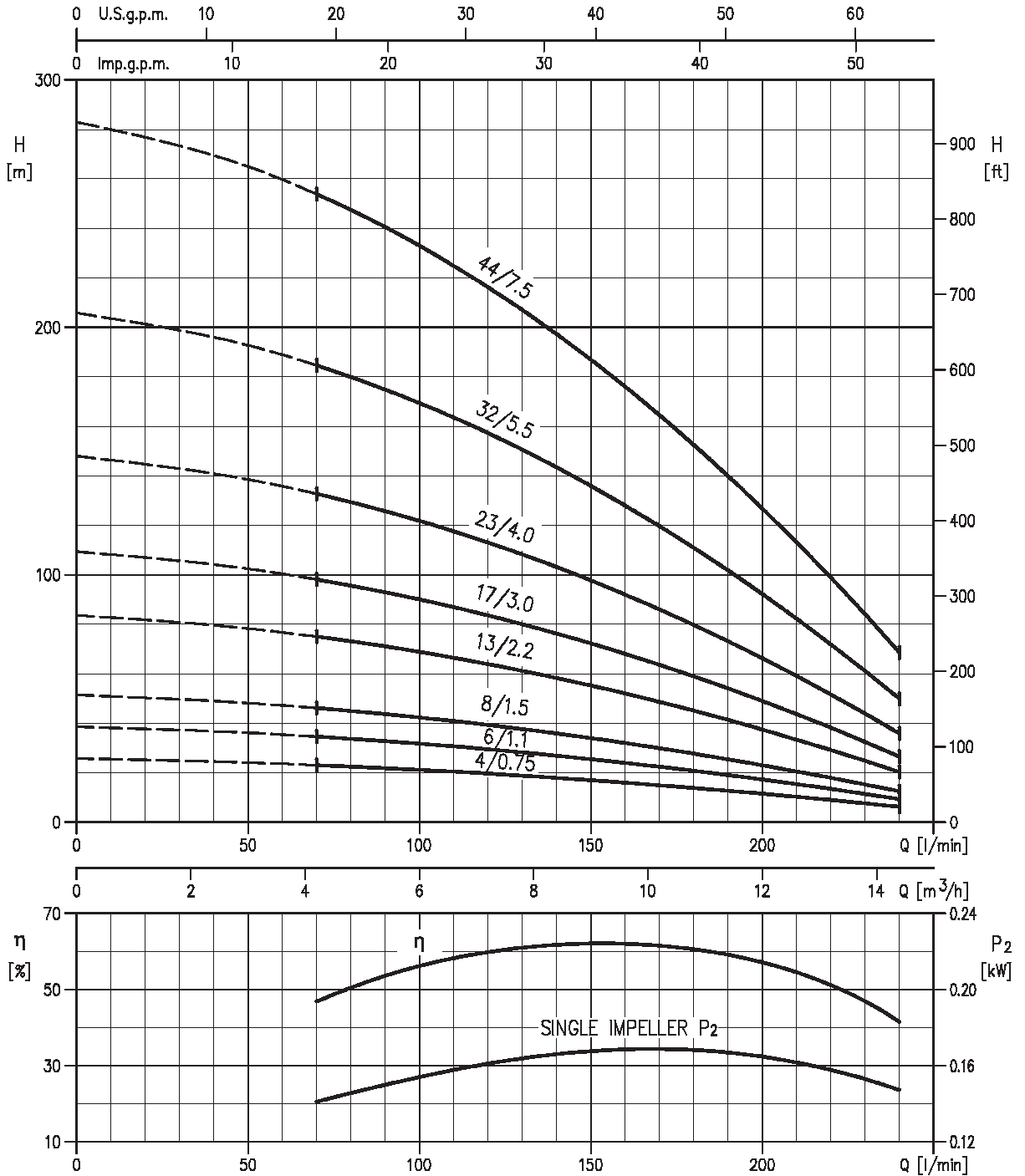
WINNER 4N10 - MEI > 0.40 - Impeller diameter = 76.4 mm
